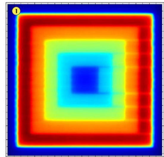
Varian MLC Pyramid Image
